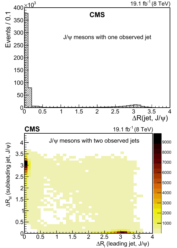
Fig. 1. The distributions of (upper) \Delta R(\text{jet}, J/\psi) for one-jet events and (lower) \Delta R_l(\text{leading jet}, J/\psi) vs. \Delta R_{sl}(\text{subleading jet}, J/\psi) for two-jet events.
