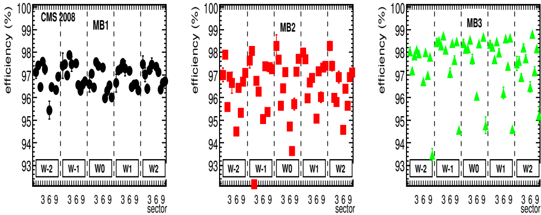
Figure 18. Segment reconstruction efficiency in the r - z planes in the barrel muon chambers, as a function of the sector number for the different wheels.
