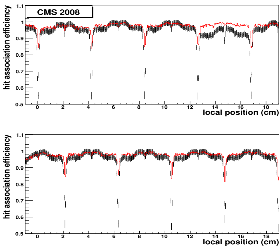
Figure 13. Efficiency for hit reconstruction and association to the muon track segment as a function of the predicted muon position in layer one (top) and layer two (bottom) of one SL in the MB2 station of sector 4 in YB0. A region corresponding approximately to four DT cells in each layer is shown. Points: data; full line histogram: simulation. Note the suppressed zero of the vertical axis.
