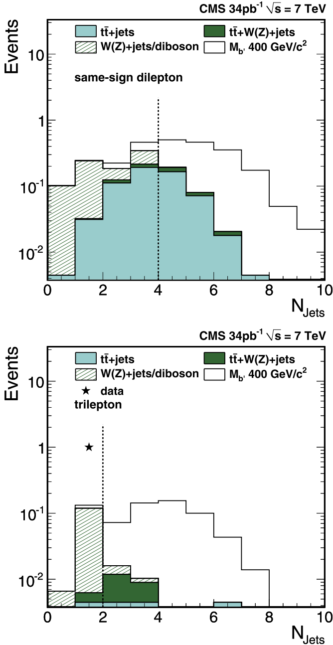
Fig. 1. Jet multiplicity distributions for the same-sign dilepton channel (top), and the tripleton channel (bottom). The star in the bottom plot represents the single measured event, which fails to satisfy the requirement on jet multiplicity. The open histogram is the signal contribution expected from a b' with M_{b'} = 400 GeV/c 2 . The light blue and dark green filled histograms show the contributions from t\bar{t} +jets and t\bar{t} +W(Z)+jets respectively. The shaded histogram represents electroweak processes (W(Z)+jets, dibosons). All selections are applied except the one corresponding to the plotted variable. The histograms are normalized to the predictions from simulation. The vertical dotted lines indicate the minimum numbers of jets required in events selected for each of the channels. (For interpretation of the references to colour in this figure legend, the reader is referred to the web version of this Letter.)
