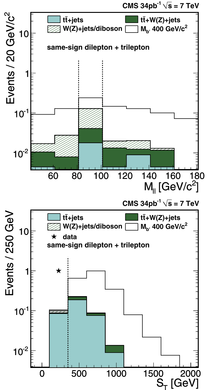
Fig. 2. The invariant mass distribution (top) of two muons with opposite charges or electrons of any charge, M(\ell\ell) , and the S_T distribution (bottom) including same-sign dilepton and tripleton channels. The star in the bottom plot represents the measured event, which fails to satisfy the requirement on S_T . The open histogram is the signal contribution expected from a b' with M_{b'} = 400 GeV/c 2 . The light blue and dark green filled histograms show the contributions from t\bar{t} +jets and t\bar{t} +W(Z)+jets respectively. The shaded histogram represents electroweak processes (W(Z)+jets, dibosons). All selections are applied except the one corresponding to the plotted variable. Events with an electron pair or an opposite sign muon pair, with M(\ell\ell) falling in the region defined by the vertical dotted lines on the top plot, are rejected in order to suppress the background from Z events. The histograms are normalized to the predictions from simulation. The vertical dotted line in the bottom plot indicates the lower S_T threshold used in the analysis. (For interpretation of the references to colour in this figure legend, the reader is referred to the web version of this Letter.)
