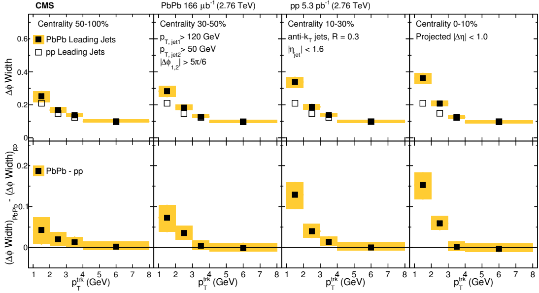
Figure 9. Comparison of the widths in PbPb and pp of the \Delta\phi charged-particle distributions correlated to leading jets with p_{T,\text{jet1}} > 120 GeV, as a function of p_T^{\text{trk}} . The bottom row shows the difference of the widths in PbPb and pp data. The shaded band corresponds to systematic uncertainty, and statistical uncertainties are smaller than symbol size.
