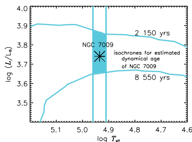
Figure 1. Region of solution is marked.
