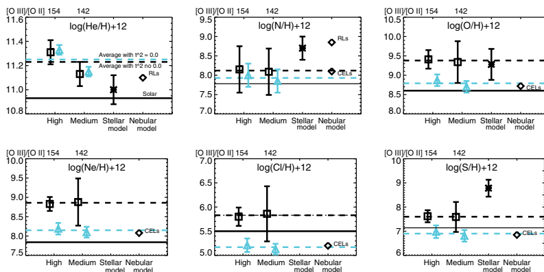
Figure 2. Comparison of the abundances in the nebular regions and models. Triangles are the abundances with t^2 = 0.00 and squares are the abundances with t^2 \neq 0.00 in the nebular regions.
