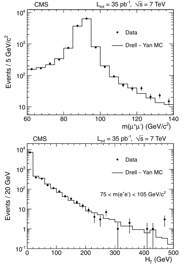
Fig. 3. Two-lepton events in data, compared with the SM simulation. Top: mass spectrum for Z \rightarrow \mu\mu . Bottom: H_T distribution for Z \rightarrow ee . Processes other than Drell-Yan are too rare to be visible in these distributions.
