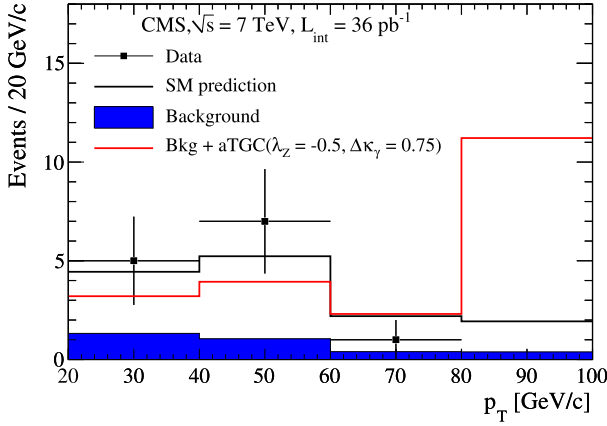
Fig. 2. Leading lepton p_T distribution in data overlaid with predictions from the SM simulation, background only simulation (Bkg in the figure) and the simulation with large anomalous couplings (aTGC in the figure).
