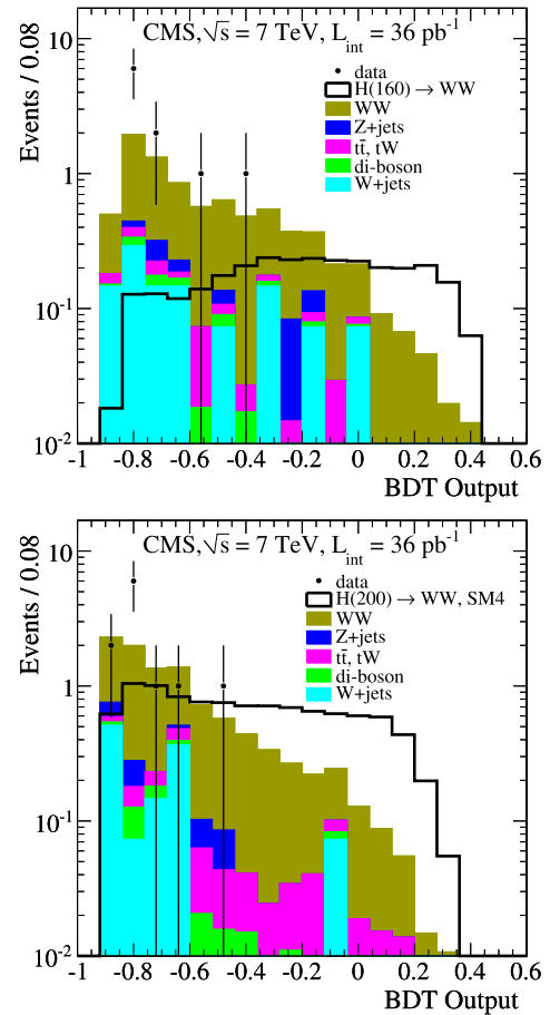
Fig. 5. BDT outputs for Higgs boson signal and for backgrounds, for (top) m_H = 160 GeV/ c^2 and (bottom) m_H = 200 GeV/ c^2 . The Higgs boson event yield is normalized (a) to the SM expectation, and (b) to the fourth family scenario. The area marked as W^+W^- corresponds to the nonresonant contribution.
