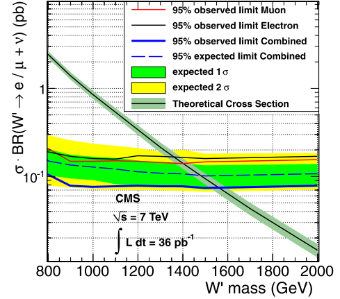
Fig. 5. Individual limits as observed for the electron (black line) and the muon channel (red line). Their combination is shown as a solid blue line for the observed limit (expected as dashed blue line), using a Bayesian technique with only the luminosity uncertainty correlated. The NNLO cross section for the considered model, including PDF uncertainties, is also shown. (For interpretation of the references to colour in this figure legend, the reader is referred to the web version of this Letter.)
