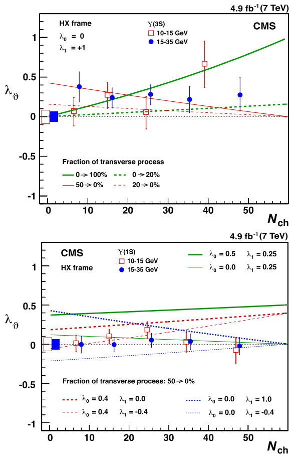
Fig. 6. Expected N_{ch} -dependences of the \lambda_{\theta} parameter for the sum of two processes, of polarizations \lambda_0 and \lambda_1 , of relative fractions changing linearly with N_{ch} (see text for details). The measured \lambda_{\theta} values are also shown, for the \Upsilon(3S) (top) and \Upsilon(1S) (bottom).
