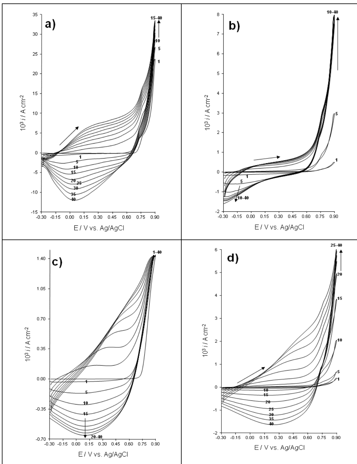
Figure 1. Cyclic voltammetry of the electropolymerization of 0.1 M Py on a vitreous carbon electrode in aqueous medium in the presence of different anions (all at 0.1 M concentration): a) \text{H}_2\text{SO}_4 , b) \text{K}_2\text{SO}_4 , c) HCl, and d) KCl. Each plot comprises 40 cycles between -0.3 and 0.9 V vs. Ag/AgCl at a scan rate = 100 mV/s.
