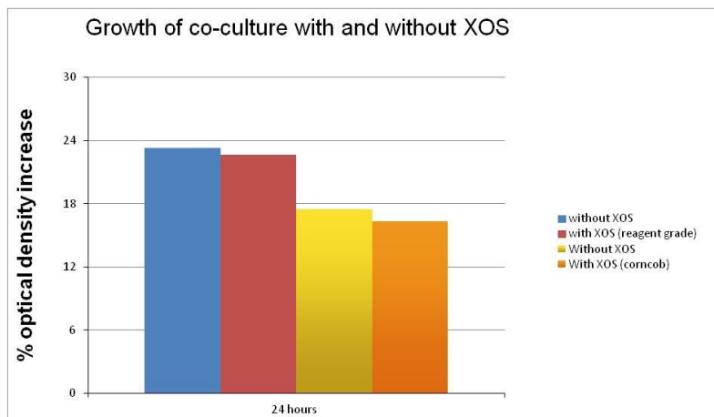
Fig. 2: Comparison of co-culture growth, with and without reagent grade and corn cob XOS.
