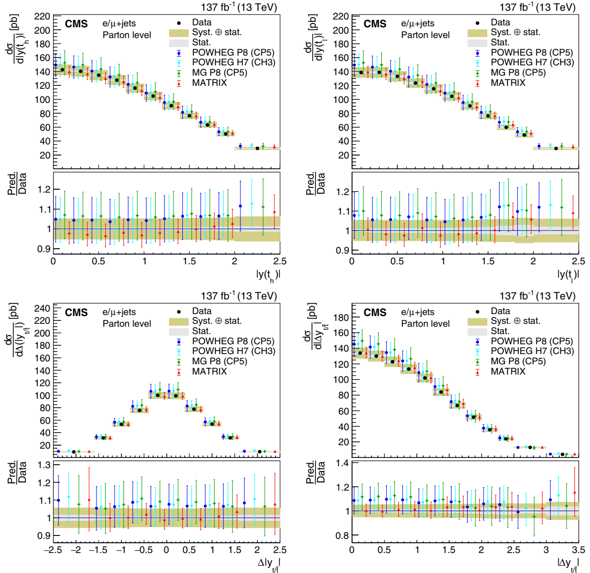
FIG. 17. Differential cross sections at the parton level as functions of |y(t_h)| , |y(t_\ell)| , and the differences \Delta|y_{l\bar{l}}| and |\Delta y_{l\bar{l}}| . The data are shown as points with gray (yellow) bands indicating the statistical (statistical and systematic) uncertainties. The cross sections are compared to the predictions of POWHEG combined with PYTHIA (P8) or HERWIG (H7), the multiparton simulation MG5_aMC@NLO (MG)+PYTHIA FxFx, and the NNLO QCD calculations obtained with MATRIX. The ratios of the various predictions to the measured cross sections are shown in the lower portion of each panel.
