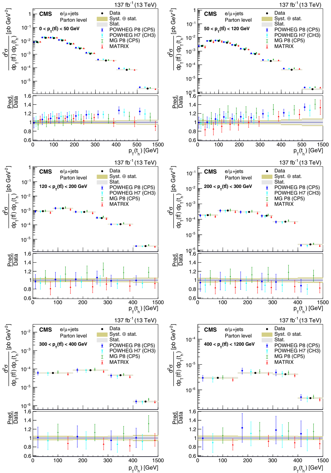
FIG. 29. Double-differential cross section at the parton level as a function of p_T(\tilde{t}) vs p_T(t_h) . The data are shown as points with gray (yellow) bands indicating the statistical (statistical and systematic) uncertainties. The cross sections are compared to the predictions of POWHEG combined with PYTHIA (P8) or HERWIG (H7), the multiparton simulation MG5_aMC@NLO (MG)+PYTHIA FxFx, and the NNLO QCD calculations obtained with MATRIX. The ratios of the various predictions to the measured cross sections are shown in the lower portion of each panel.
