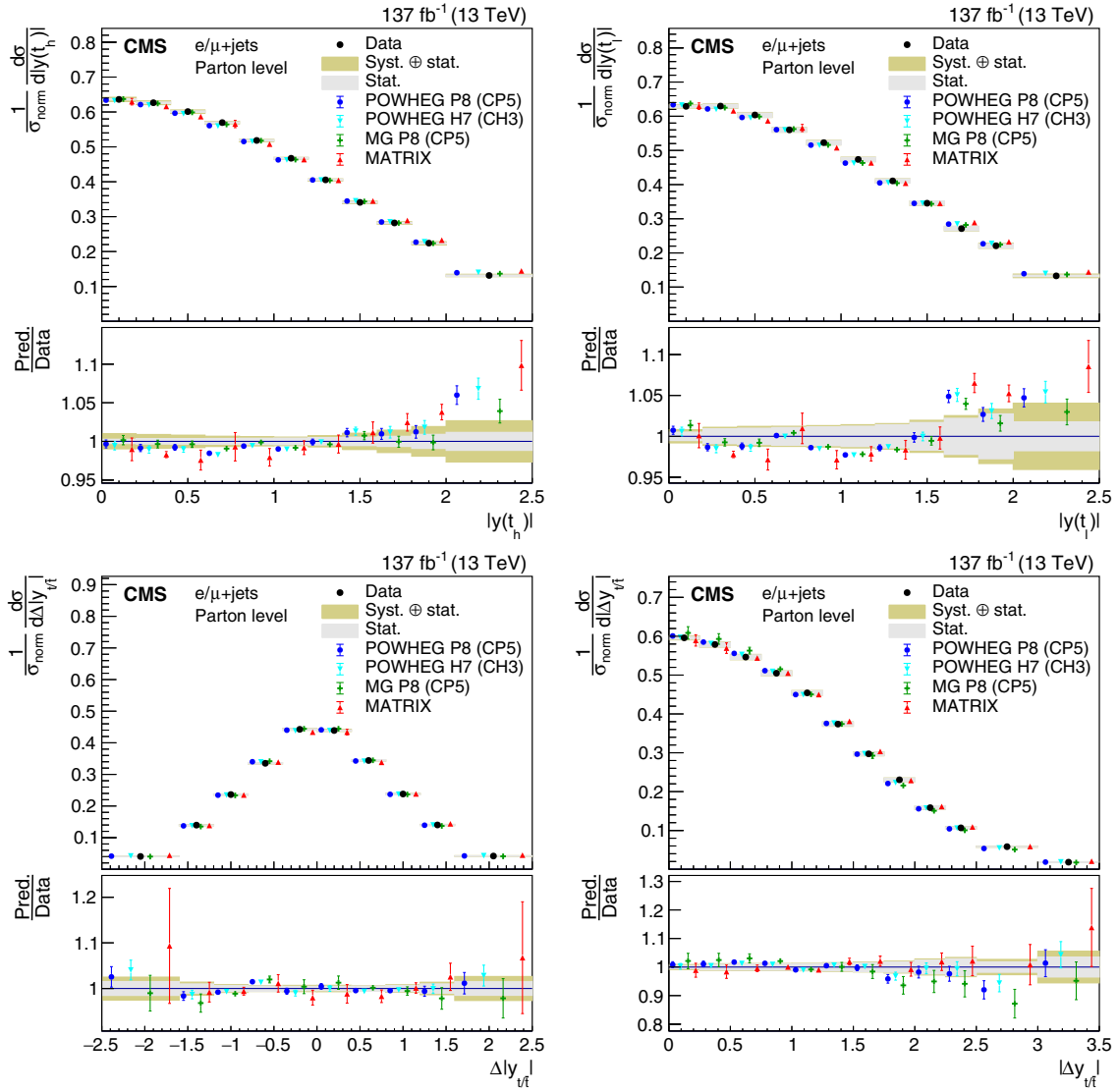
FIG. 45. Normalized differential cross sections at the parton level as functions of |y(t_h)| , |y(t_\ell)| , and the differences |\Delta y_{t\ell}| and |\Delta y_{t\ell}| . The data are shown as points with gray (yellow) bands indicating the statistical (systematic) uncertainties. The cross sections are compared to the predictions of POWHEG combined with PYTHIA (P8) or HERWIG (H7), the multiparton simulation MG5_aMC@NLO (MG)+PYTHIA FxFx, and the NNLO QCD calculations obtained with MATRIX. The ratios of the various predictions to the measured cross sections are shown in the lower portion of each panel.
