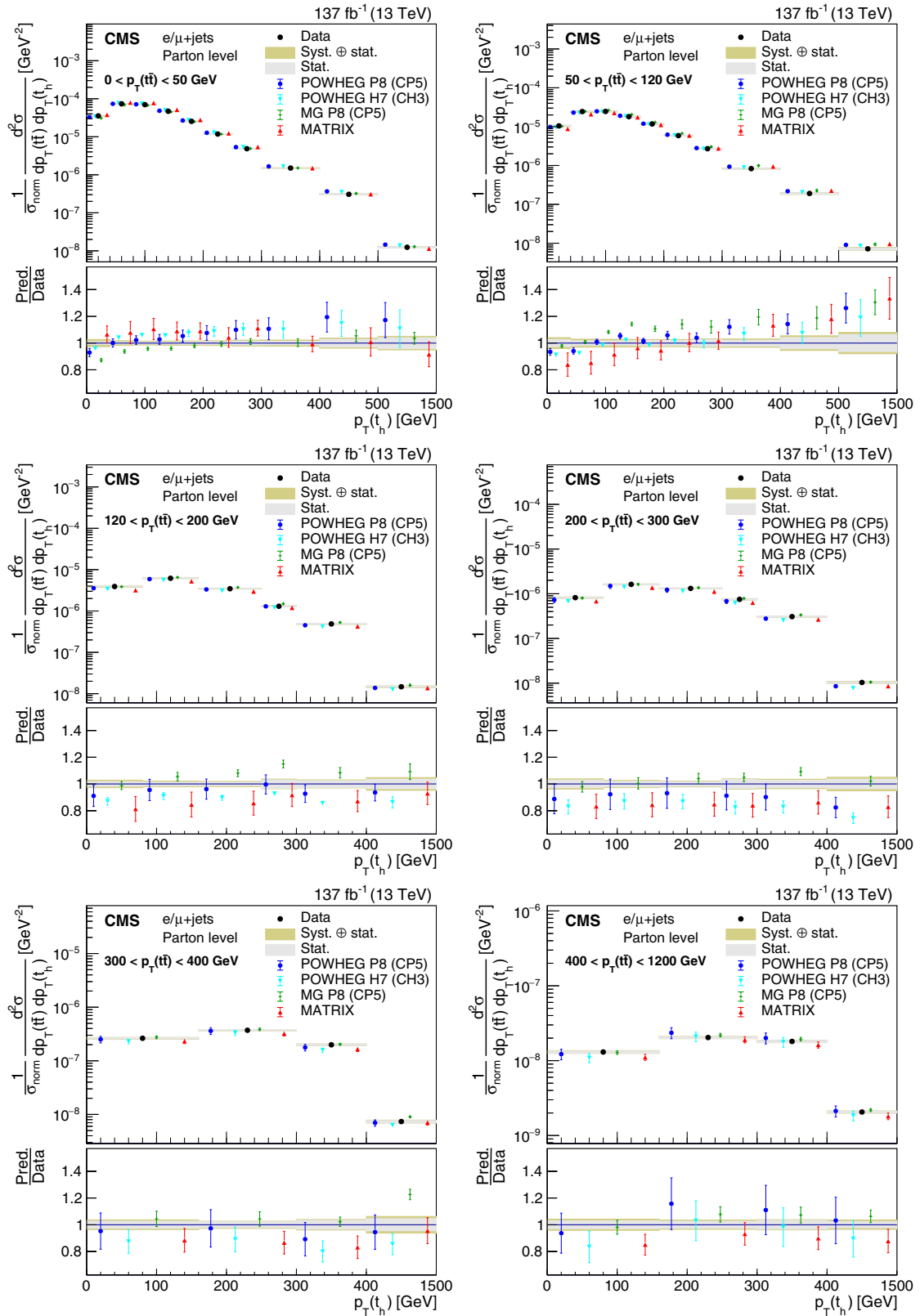
FIG. 57. Normalized double-differential cross section at the parton level as a function of p_T(\tilde{t}\bar{\tilde{t}}) vs p_T(t_h) . The data are shown as points with gray (yellow) bands indicating the statistical (statistical and systematic) uncertainties. The cross sections are compared to the predictions of POWHEG combined with PYTHIA (P8) or HERWIG (H7), the multiparton simulation MG5_aMC@NLO (MG)+PYTHIA FxFx, and the NNLO QCD calculations obtained with MATRIX. The ratios of the various predictions to the measured cross sections are shown in the lower portion of each panel.
