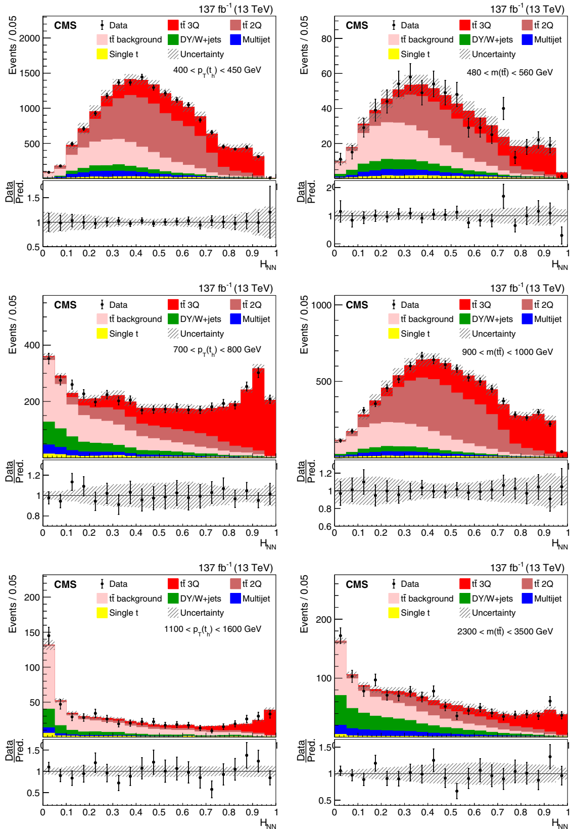
FIG. 9. The postfit H_{NN} distributions in bins of p_T(t_h) (left) and m(t\bar{t}) (right) for the data (points) and simulation (colored histograms). The electron and muon events and all three years of data taking have been combined. The hatched area shows the total uncertainties from the fit. The vertical bars on the points represent the statistical uncertainty in the data. The ratio of the data to the sum of the fitted yields is provided in the lower portion of each panel.
