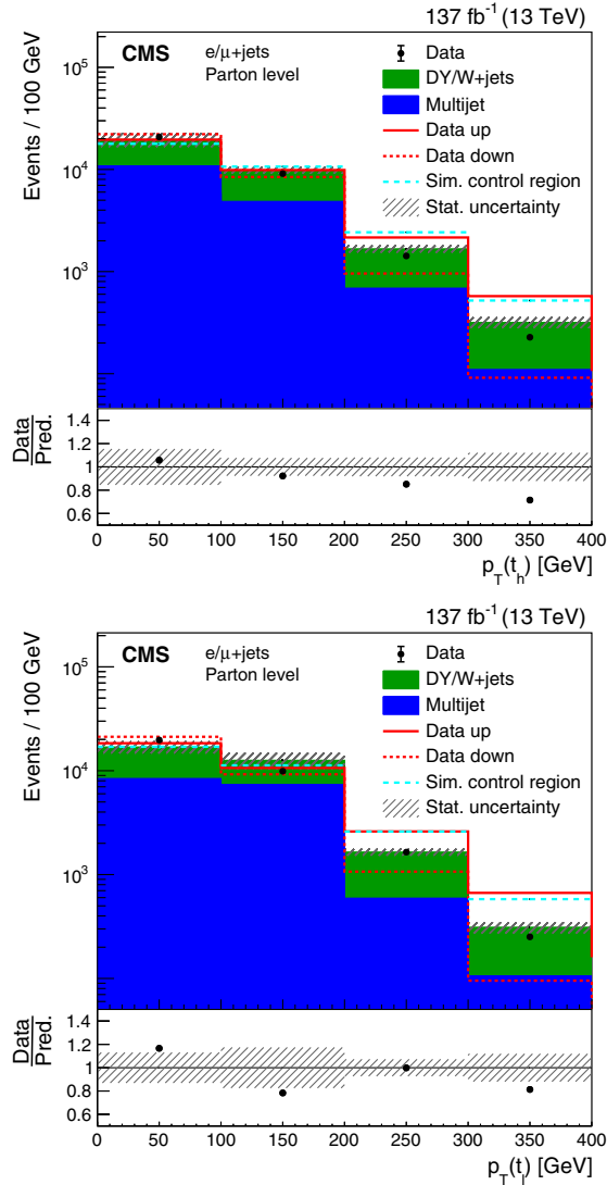
FIG. 8. The p_T(t_h) (upper) and p_T(t_e) (lower) distributions for the multijet and DY/W-boson backgrounds from data (points) in the control region and from simulation (colored histograms) in the signal region for the 1t1l category. The red lines show the variations in the control region distribution when shifting the discriminant selection range up (solid lines) and down (dotted lines). The blue dashed line gives the sum of the multijet and DY/W-boson predictions in the control region. The hatched band shows the statistical uncertainties in the prediction. The data points are shown with statistical uncertainties. The ratio of the data to the predicted yields is provided in the lower portion of each panel.
