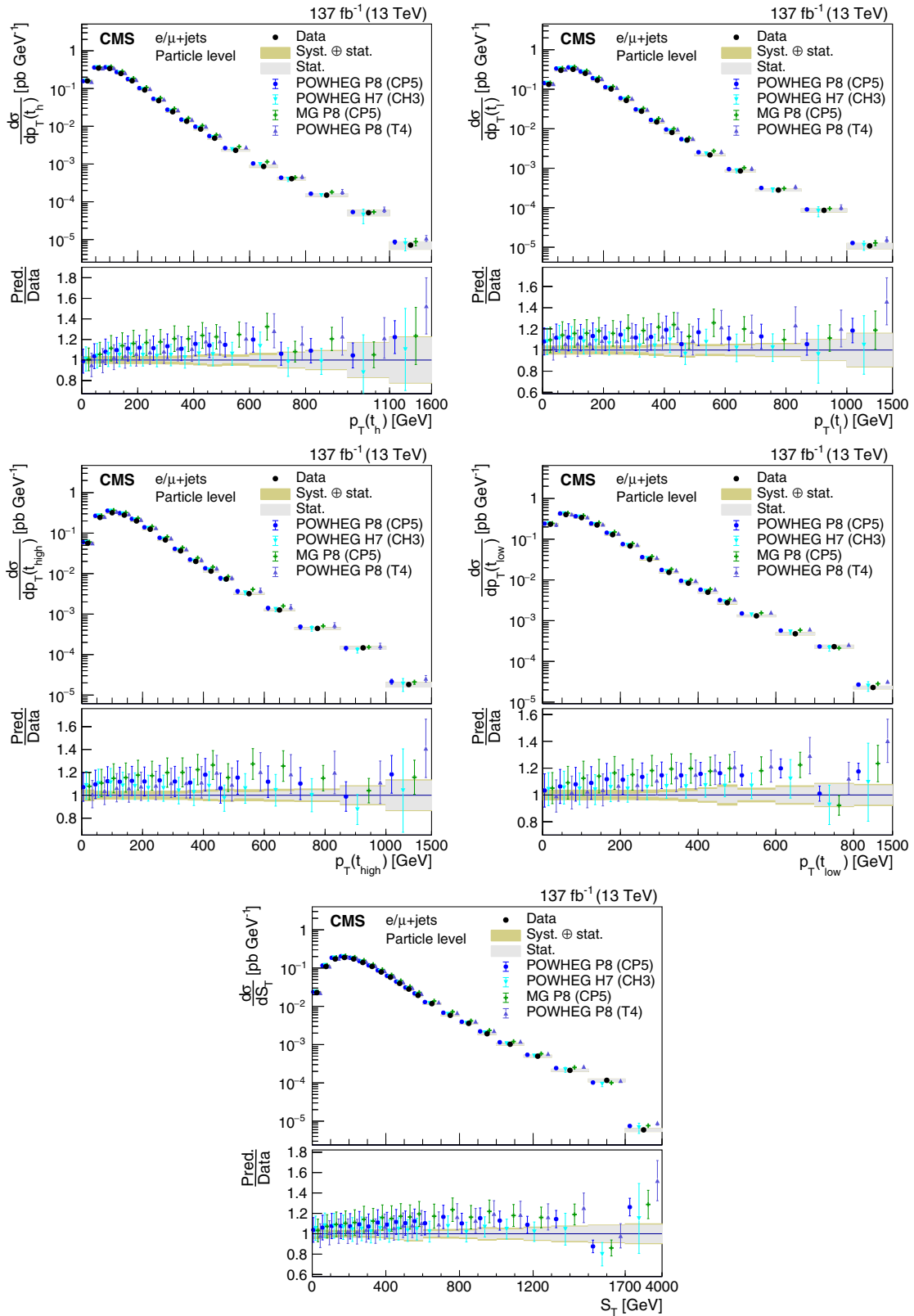
FIG. 16. Differential cross sections at the particle level as functions of p_T(t_h) , p_T(t_\ell) , p_T(t_{\text{high}}) , p_T(t_{\text{low}}) , and S_T . The data are shown as points with gray (yellow) bands indicating the statistical (statistical and systematic) uncertainties. The cross sections are compared to the predictions of POWHEG+PYTHIA (P8) for the CP5 and CUETP8M2T4 (T4) tunes, POWHEG+HERWIG (H7), and the multiparton simulation MG5_aMC@NLO (MG)+PYTHIA. The ratios of the various predictions to the measured cross sections are shown in the lower portion of each panel.
