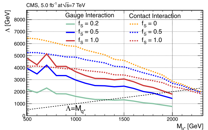
Fig. 4. Contours of excluded parameters for the gauge and contact interaction q^* production mechanisms. For a given f_s assumption, each (M_{q^*}, \Lambda) below the limit curve is excluded. The bump in the \Lambda contour at M_{q^*} = 700 GeV for the gauge interaction production models is a direct consequence of the downward fluctuation on the upper limit on the cross section observed at M_{q^*} = 700 GeV (Fig. 3).
