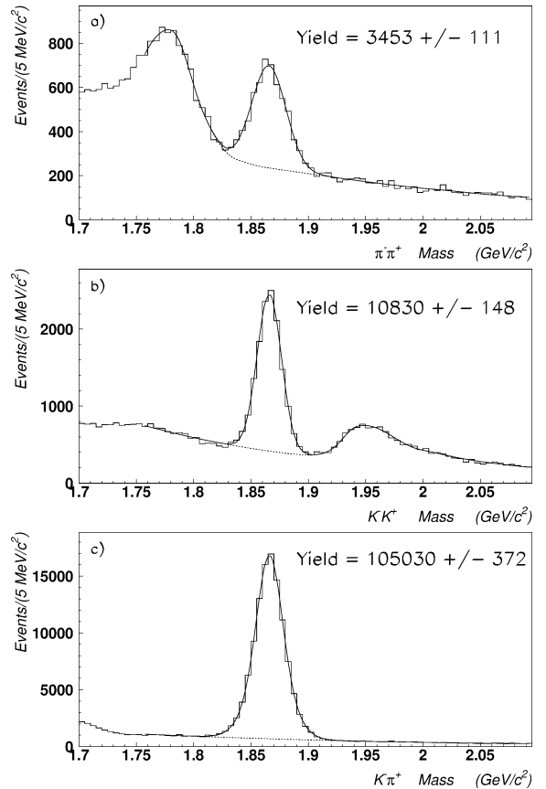
Fig. 1. Invariant mass distribution for \pi^- \pi^+ (a), K^- K^+ (b) and K^- \pi^+ (c). The fit (solid curve) for the Cabibbo-suppressed decay modes of D^0 is to a Gaussian over a polynomial (for the combinatorial background) and a function obtained with Monte Carlo simulations for the reflection peak.
