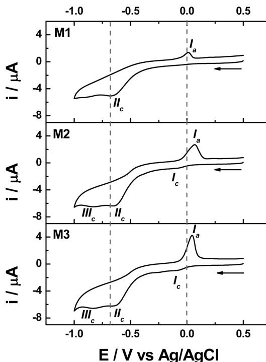
Fig. 2. Direct (non-diluted) potentiodynamic reduction of three commercial mezcal samples in the presence of 0.1 M of LiClO 4 , \nu = 25 mV/s. The first cycle is shown.
