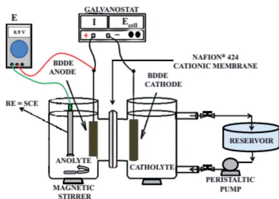
Figure 2. Electrochemical system with a divided H-type cell.
